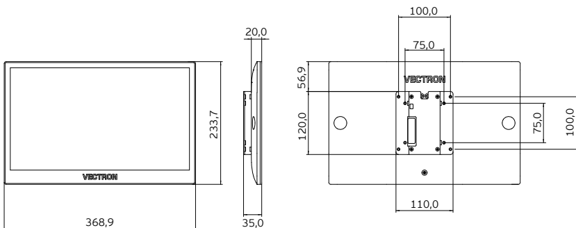
Abb. 8: Bedienerdisplay Vectron POS 7 VESA an VESA Mount Adapter
